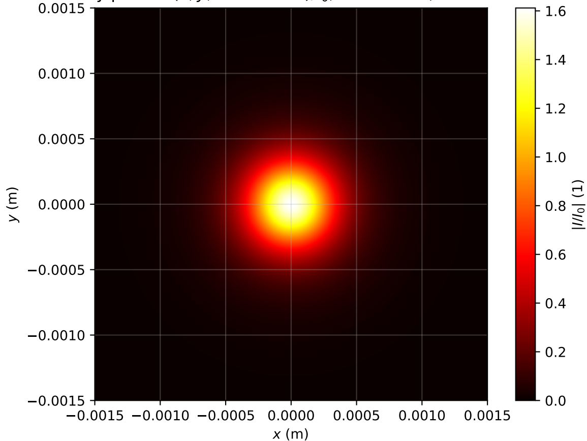
Intensity profile I(x, y, z = 1.751m)/I_0 , Pin=0.9Pcr, artificial time
